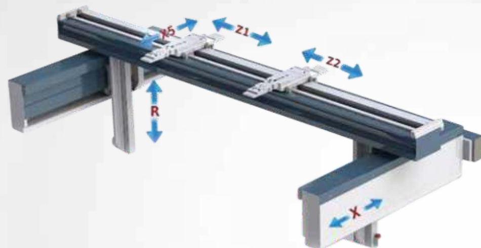
Work zone detail
