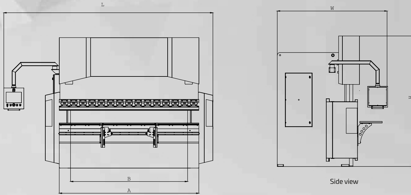
Front view
